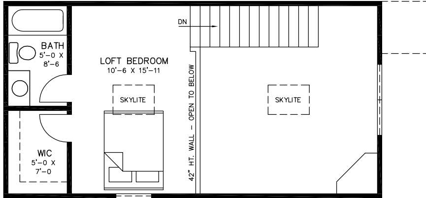
UPPER FLOOR - A SINGLE BR
