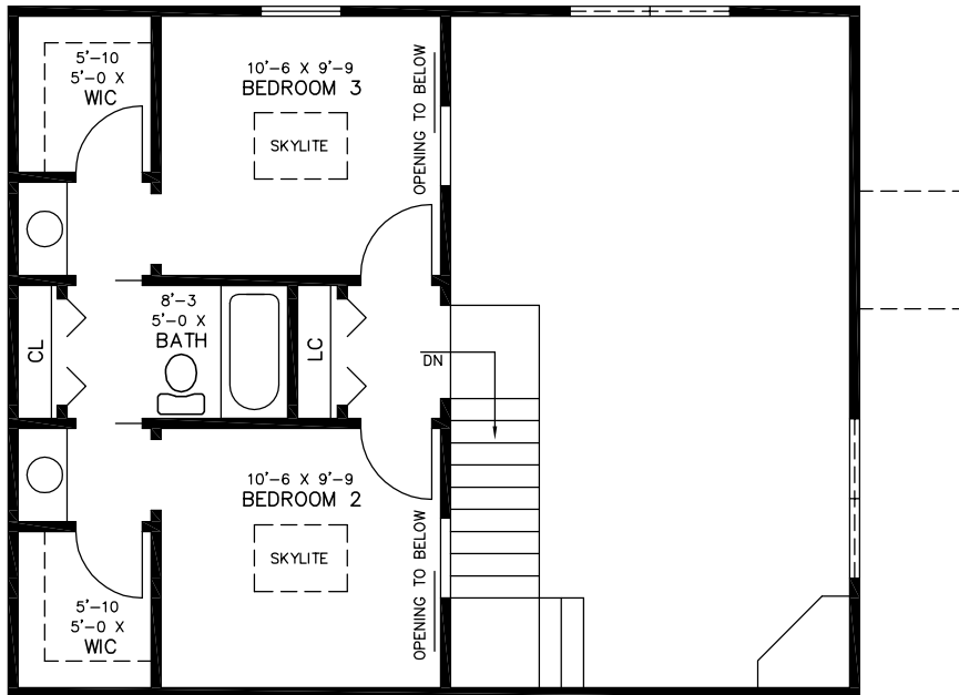
UPPER FLOOR - B THREE BR
