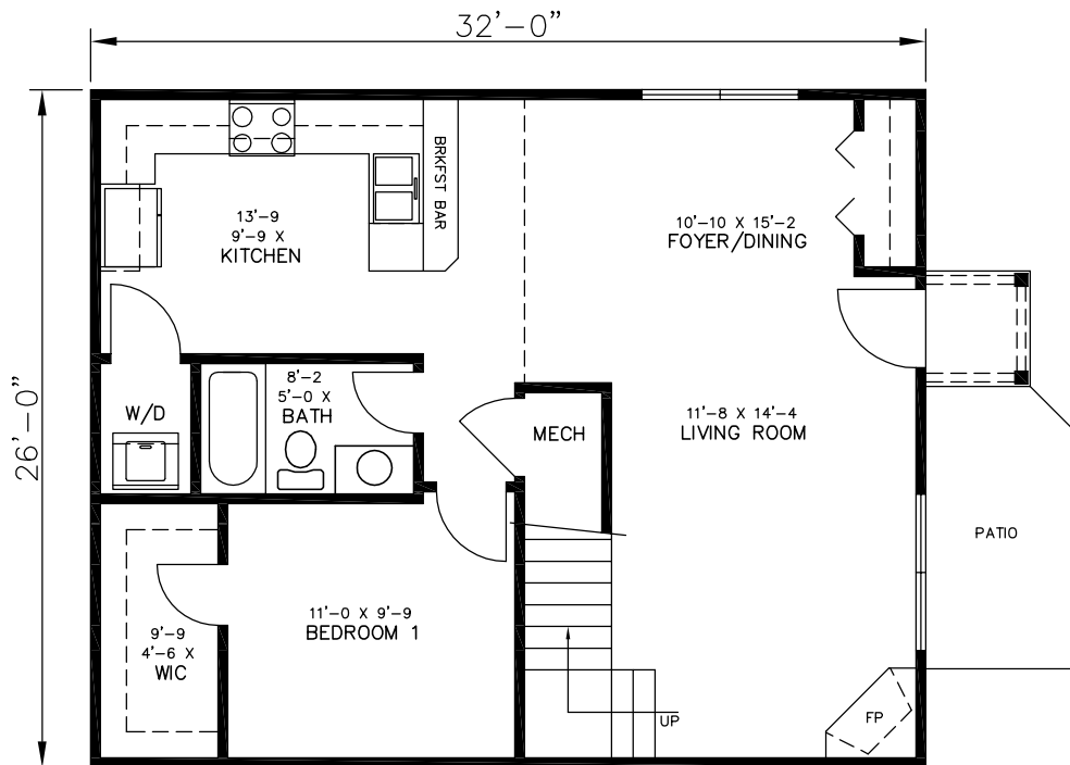
MAIN FLOOR - B THREE BR
